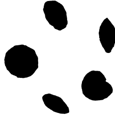
FIG. 71.—COLONIES ON NUTRIENT AGAR-AGAR, \times 60 .
